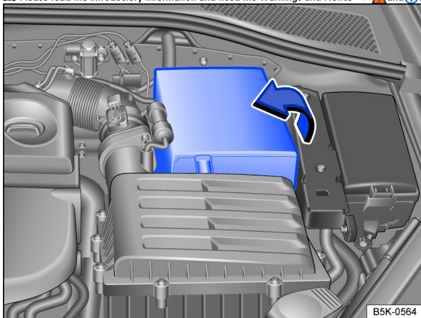
Fig. 198 Open the cover on the 12-volt vehicle battery in the engine compartment.
