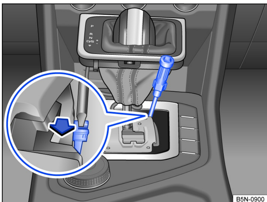
Fig. 121 Manually release the selector lever lock.
