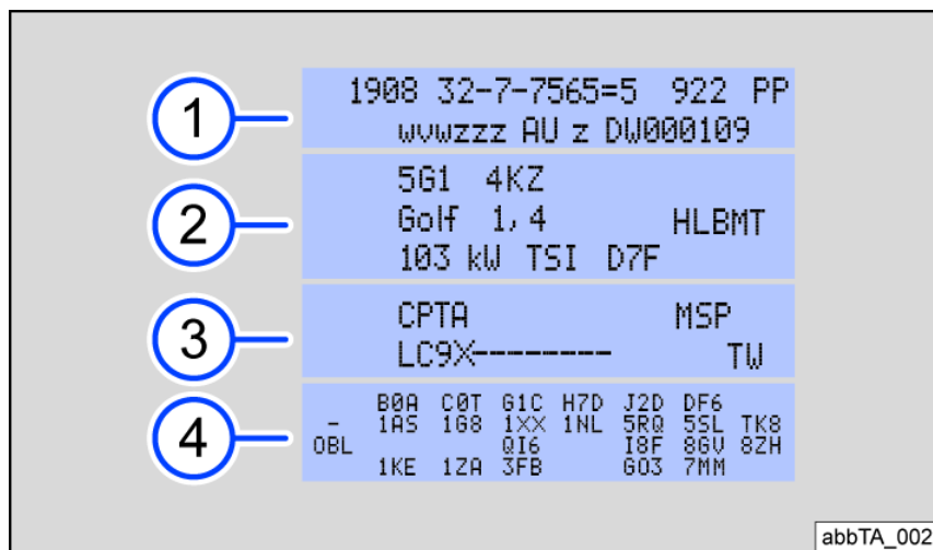
Fig. 218 General example: vehicle data label
