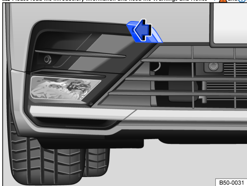
Fig. 185 In the front right bumper: Cap for the towing eye mounts.
