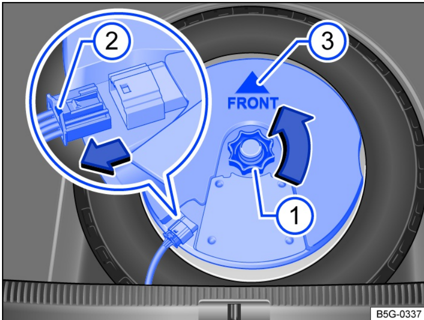
Fig. 209 In the luggage compartment: removing the subwoofer (version 2).
