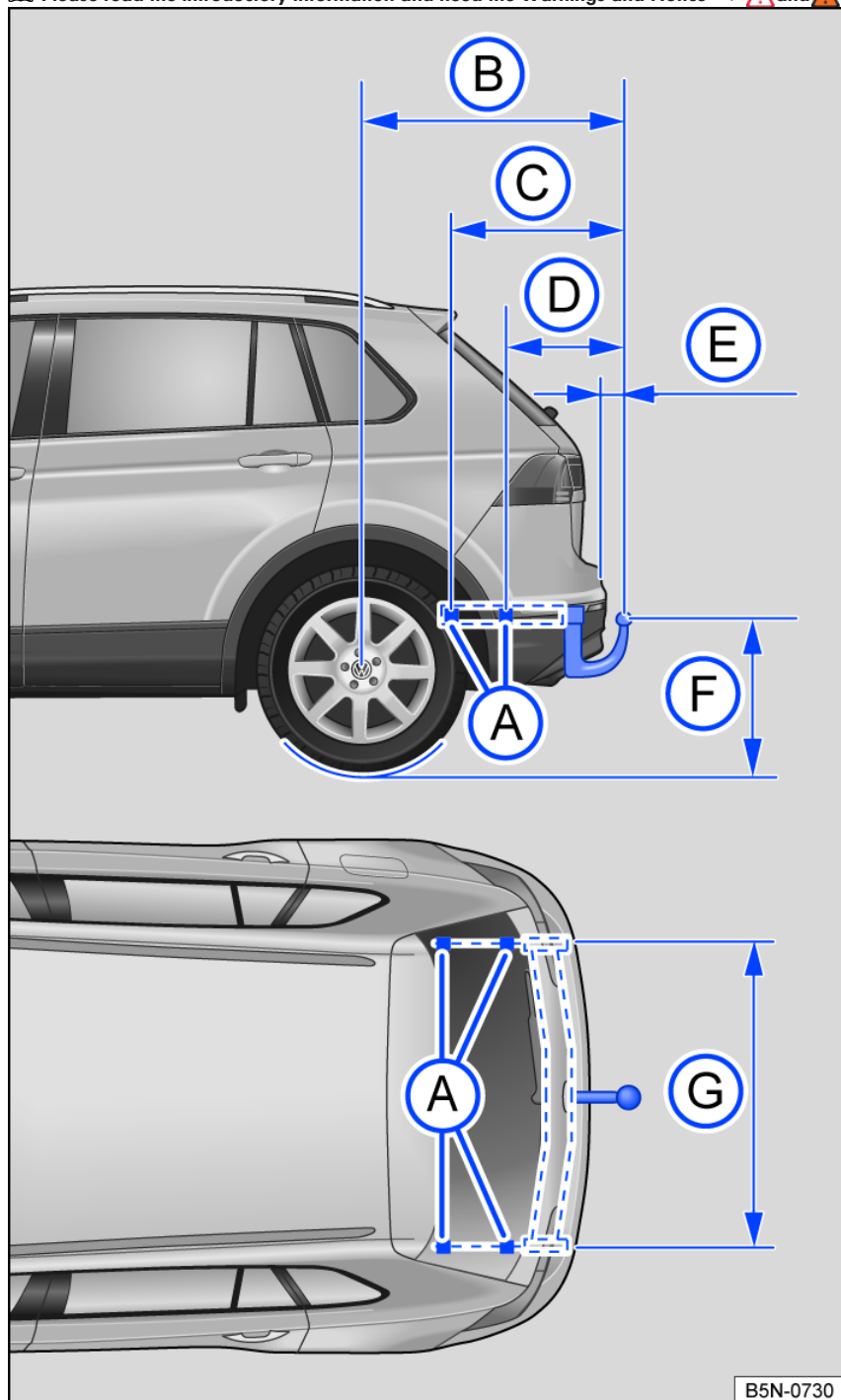
Fig. 163 Dimensions and mounting points for retrofitting a trailer hitch.
