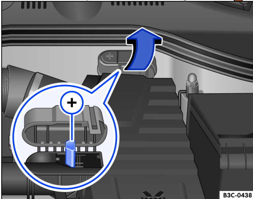
Fig. 181 Located in the engine compartment under a cover: Jump-starting point (positive battery terminal).
