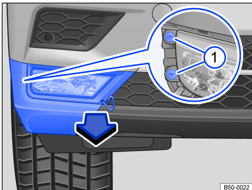
Fig. 171 In the right side of the front bumper: removing the fog lights.
