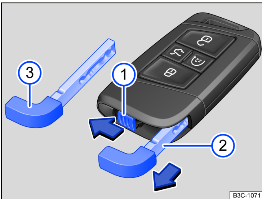
Fig. 50 Vehicle key: releasing the mechanical key.
