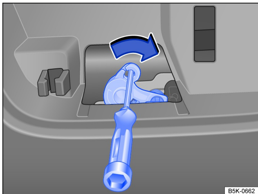
Fig. 70 In the trunk lid: emergency release for the trunk lid.
