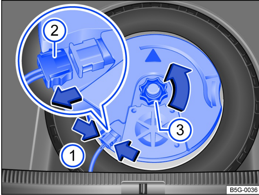
Fig. 208 In the luggage compartment: removing the subwoofer (version 1).
