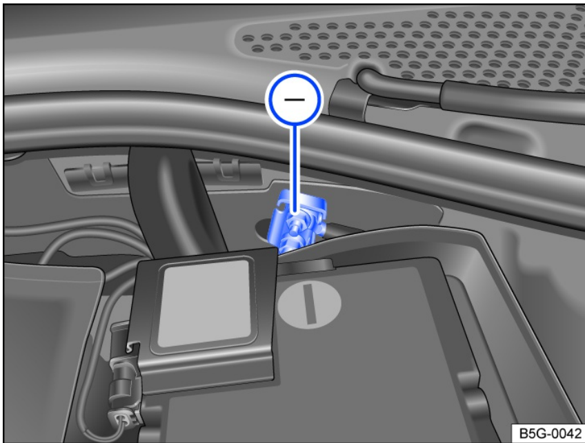
Fig. 182 In the engine compartment: jump-start point (negative connection).
