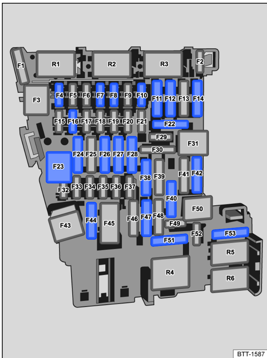
Fig. 178 Fuse assignment in the instrument panel.
