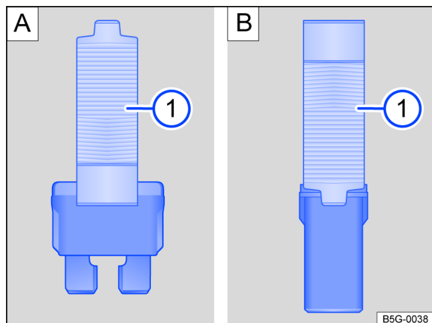
Fig. 180 Removing or installing a fuse with the plastic pliers: A : flat connector fuse, B : block fuse.
