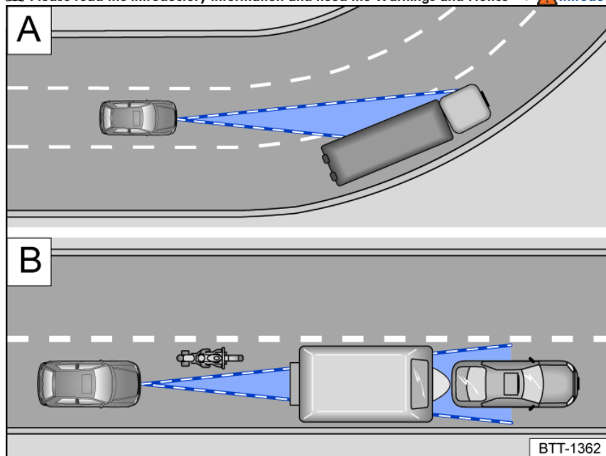
Fig. 129 A Driving around curves. B Vehicles outside of the radar sensor range.
