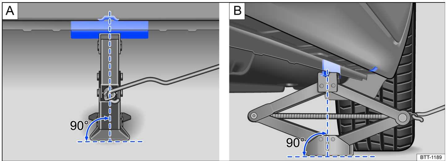
Fig. 212 Jack positioned on the left rear side of the vehicle.
