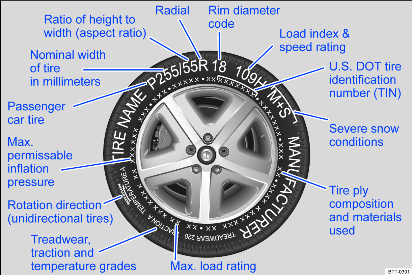
Fig. 203 International tire labeling.
