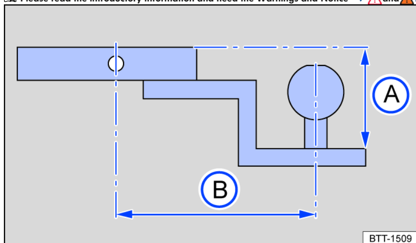
Fig. 162 Dimensions of the hitch ball holder and mount.
