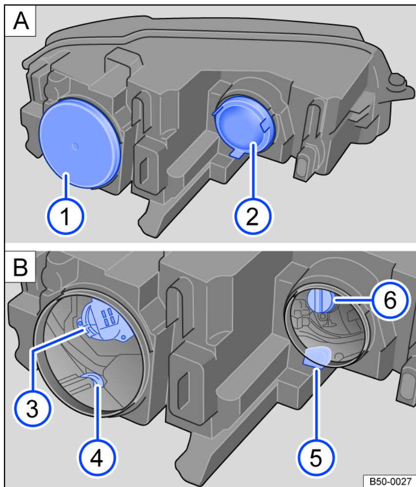
Fig. 170 In the engine compartment: A covers and B bulbs in the left headlight.
