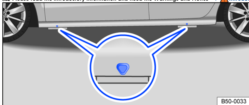
Fig. 211 Mounting points for the vehicle jack.
