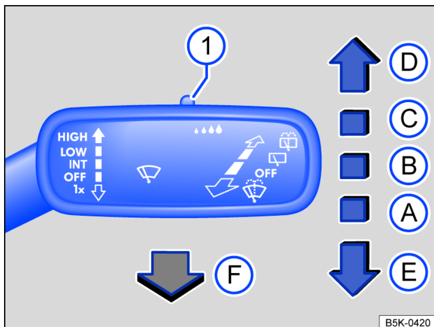
Fig. 99 On the right side of the steering column: operating the windshield wipers.
